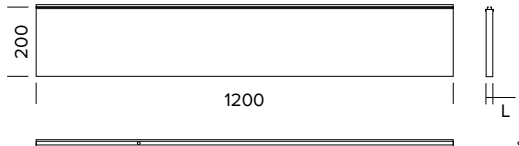
Simple Rectangle Baffle 1200/200
