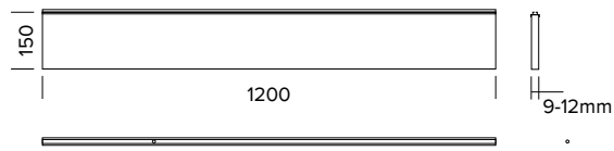
Simple Rectangle Baffle 1200/150
