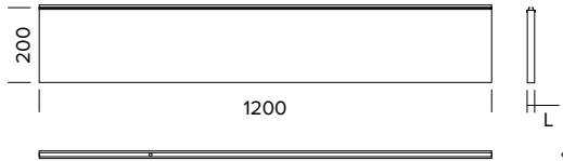
Simple Rectangle Baffle 1200/200
